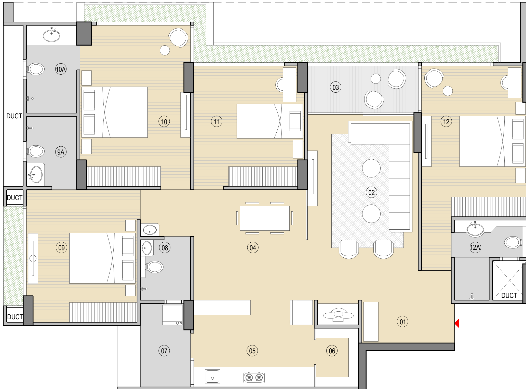
Type-B_N 4BHK_ Net area 140.51 sq.mt
