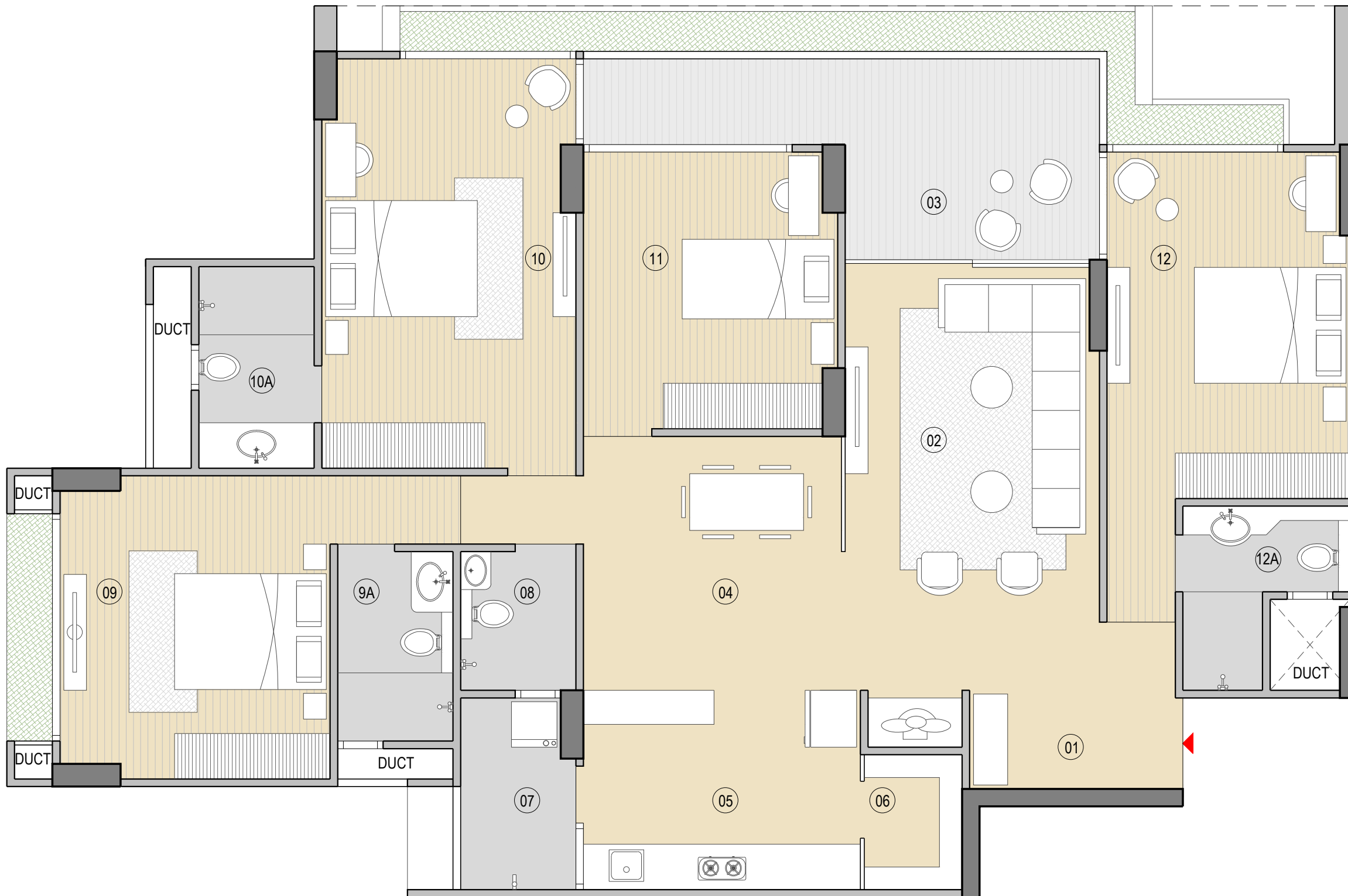
Type-A_8th & 9th floor 4BHK_Net area 153.21 sq.mt
