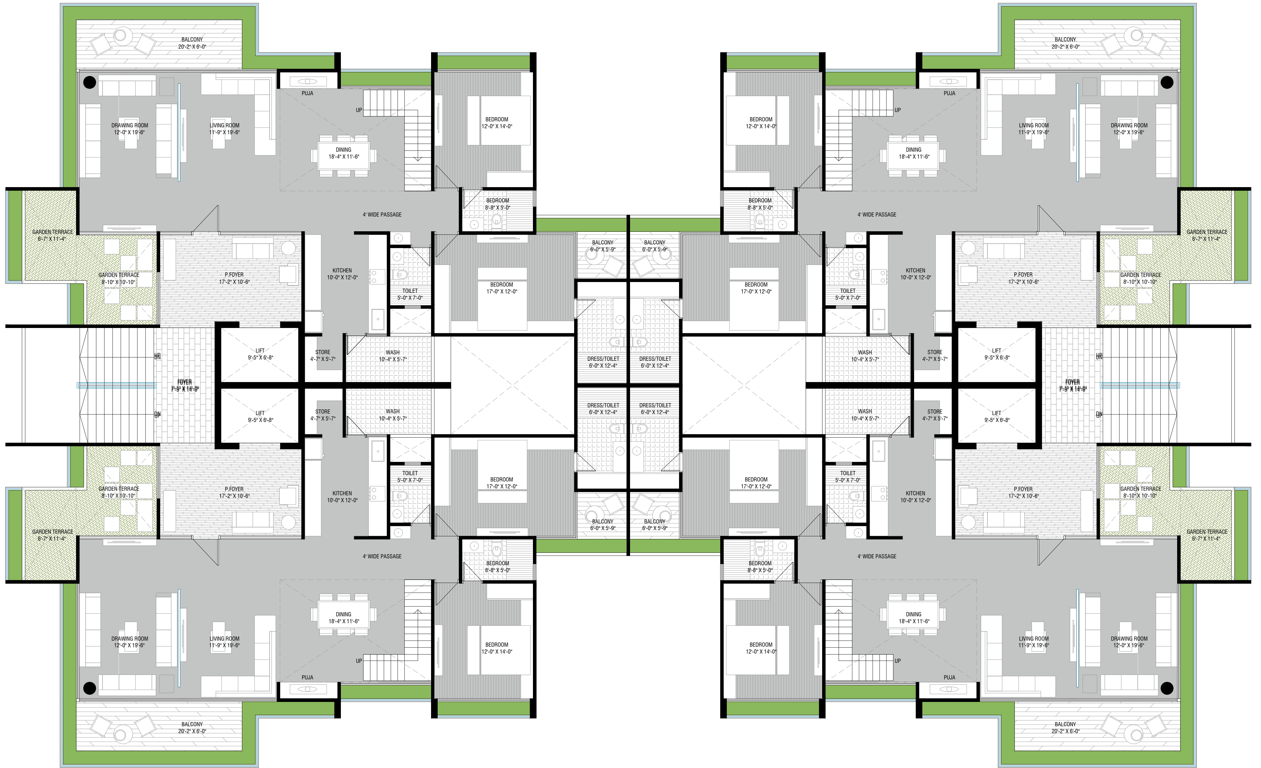
LOWER PENTHOUSE BLOCK C - D
